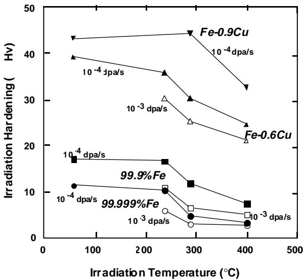
Fig. 3 Temperature dependence of irradiation hardening at 0.2 dpa for 2 levels of dose rates.
