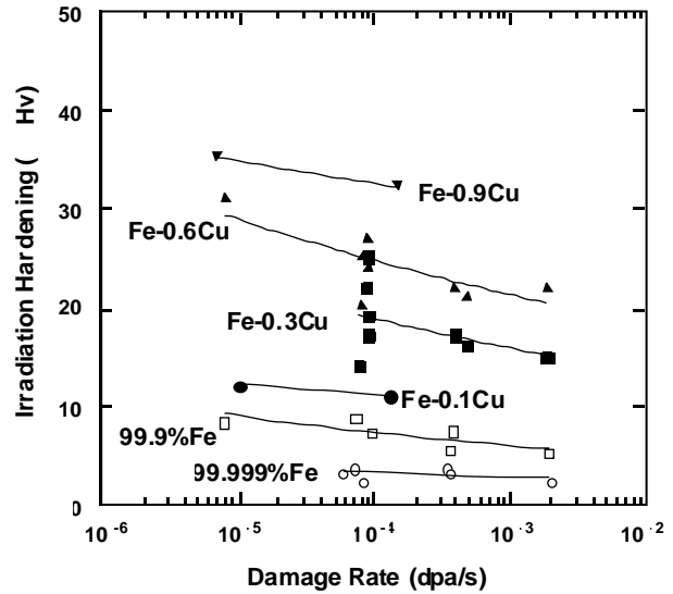
Fig. 2 Dose rate dependence of irradiation hardening at 0.2 dpa at 400°C.
