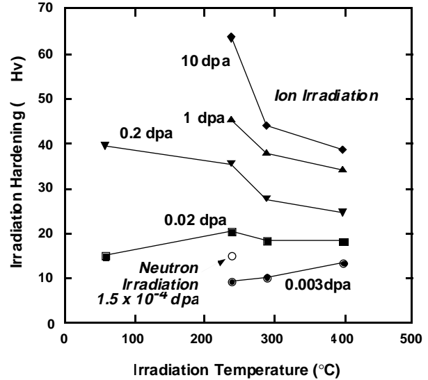
Fig. 4 Irradiation hardening in Fe-0.6Cu at several doses.
