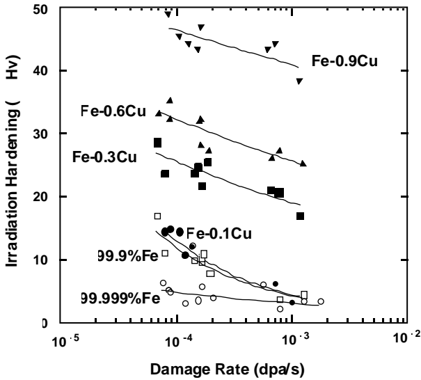
Fig. 1 Dose rate dependence of irradiation hardening at 0.2 dpa at 290°C.
